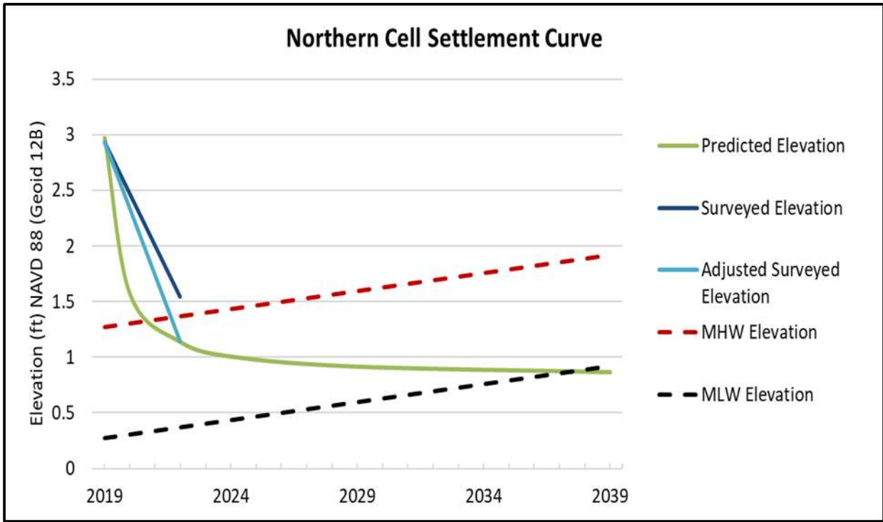
Figure 5: Predicted settlement curve and actual settlement for the CS-54 Northern Marsh Creation Cell. Adjusted surveyed elevation is adjusted for an estimated 0.4 ft of soil deposition due to Hurricanes Laura and Delta based on reference CRMS sites.
