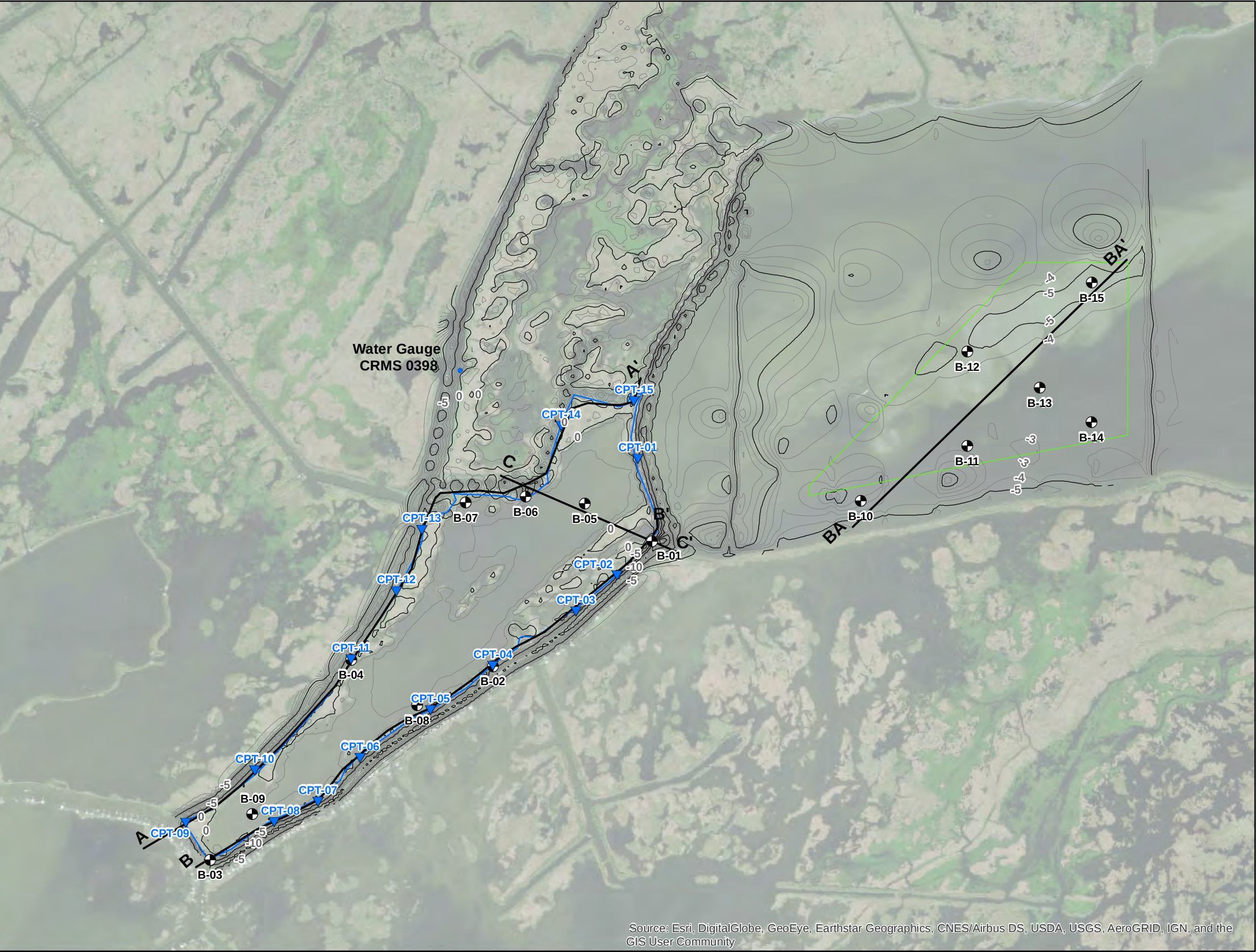
SITE LAYOUT AND EXPLORATION PLAN Bayou Decade Marsh Creation and Ridge Restoration Terrebonne Parish, Louisiana
