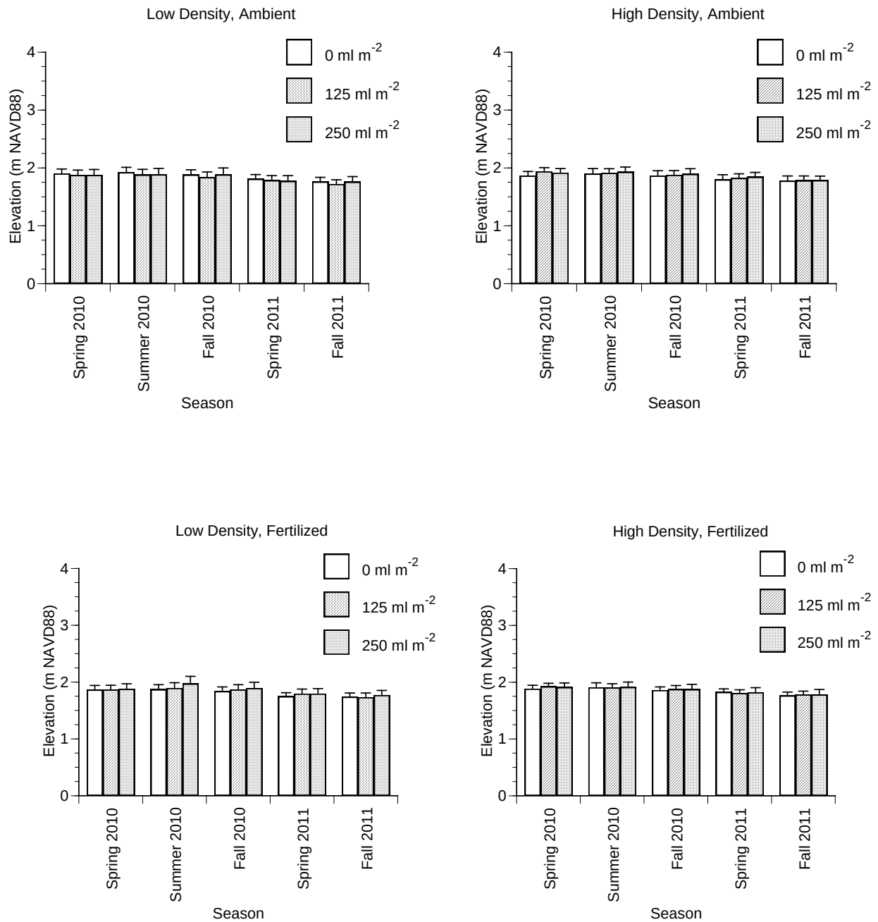
Figure 5.20 The effect of season, planting density, fertilizer regime, and humic acid amendment on Spartina patens plot elevation (m; mean \pm SE, n = 5 , Sp 2010 LSD = 0.297, Su 2010 LSD = 0.250, Fa 2010 LSD = 0.254, Sp 2011 LSD = 0.229, Fa 2011 LSD = 0.200).
