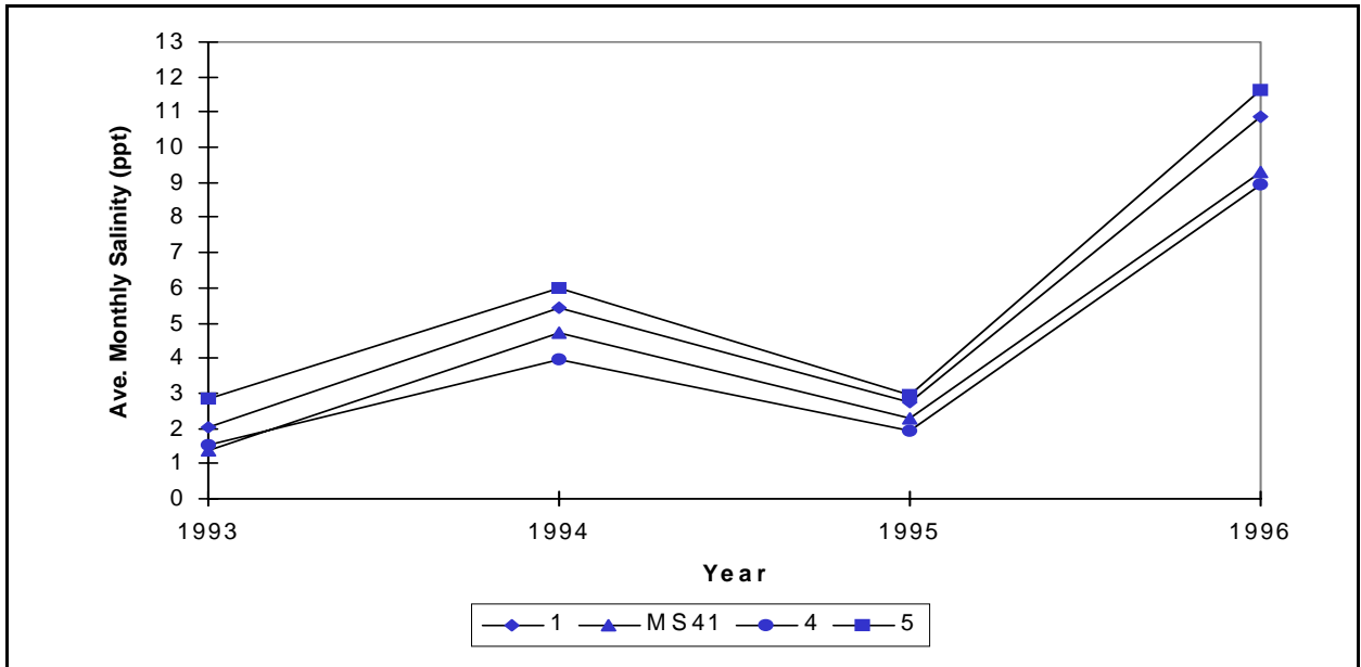
Figure 6. Average monthly salinity from January through October for years 1993 through 1996 in the West Hackberry Plantings project area at stations 1, MS41, 4, and 5. (Based on monthly and bimonthly discrete data collected by LDNR/CRD for the Rycade Canal [C/S-02] project.)
