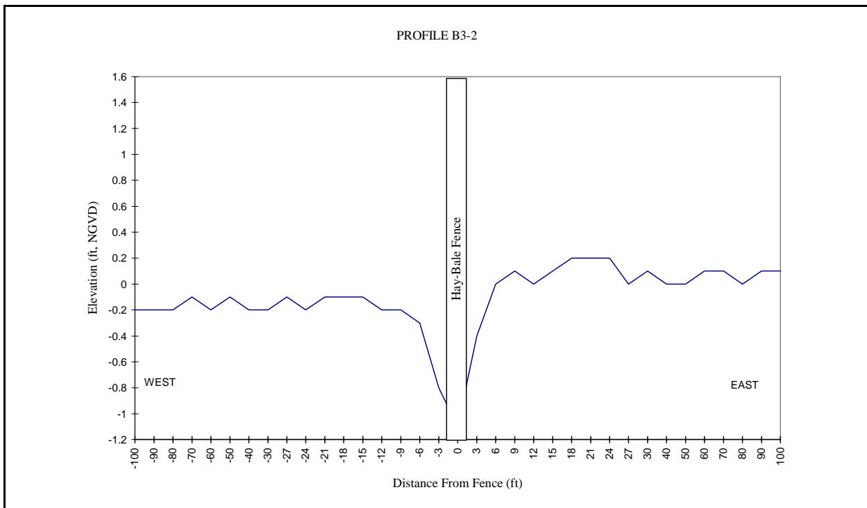
Figure 2. Elevational profile transects 1 and 2 across hay-bale fence B3 in the West Hackberry Plantings and Sediment Enhancement project area, Cameron Parish, Louisiana, surveyed August 1994. (See figure 1 for locations of fence and transects).
