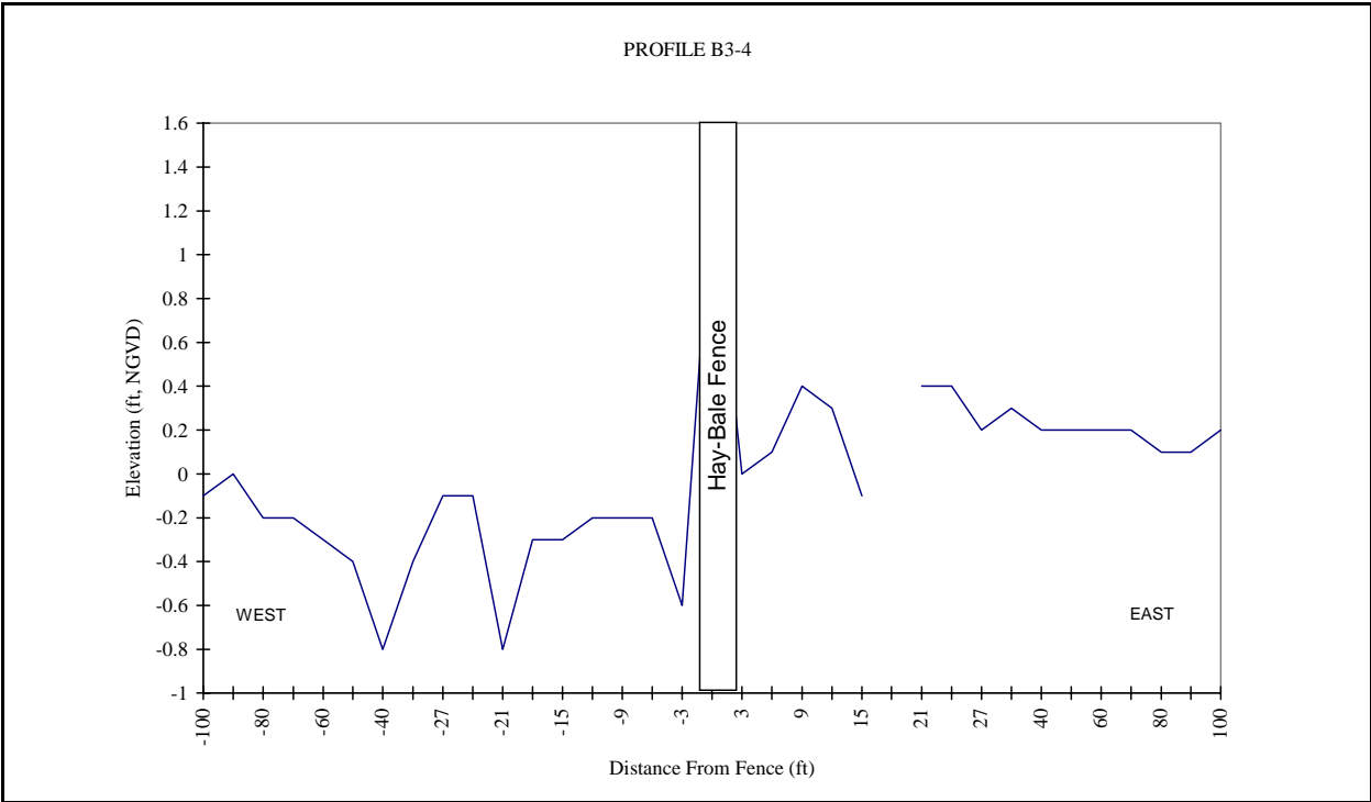
Figure 3. Elevational profile transects 3 and 4 across hay-bale fence B3 in the West Hackberry Plantings and Sediment Enhancement project area, Cameron Parish, Louisiana, surveyed August 1994. (See figure 1 for locations of fence and transects).
