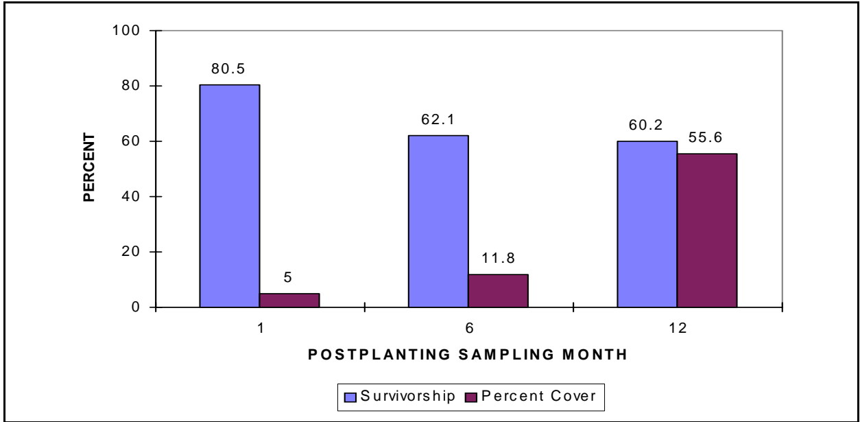
Figure 5. Mean survivorship and percent cover of S. californicus plantings in 13 random sampling plots, from August 1994 to July 1995, as observed at 1, 6, and 12 mo postplanting. (Note: only the 13 plots for which percent cover data was available at 6 and 12 mo postplanting are included in this graph).
