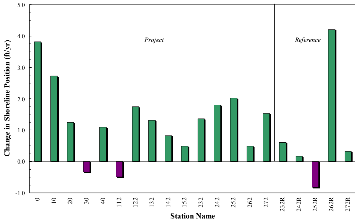
Figure 5. Sabine Refuge Protection (CS-18) shoreline change for the project and reference area from 1995 to 2000. Rates are calculated in ft/yr.
