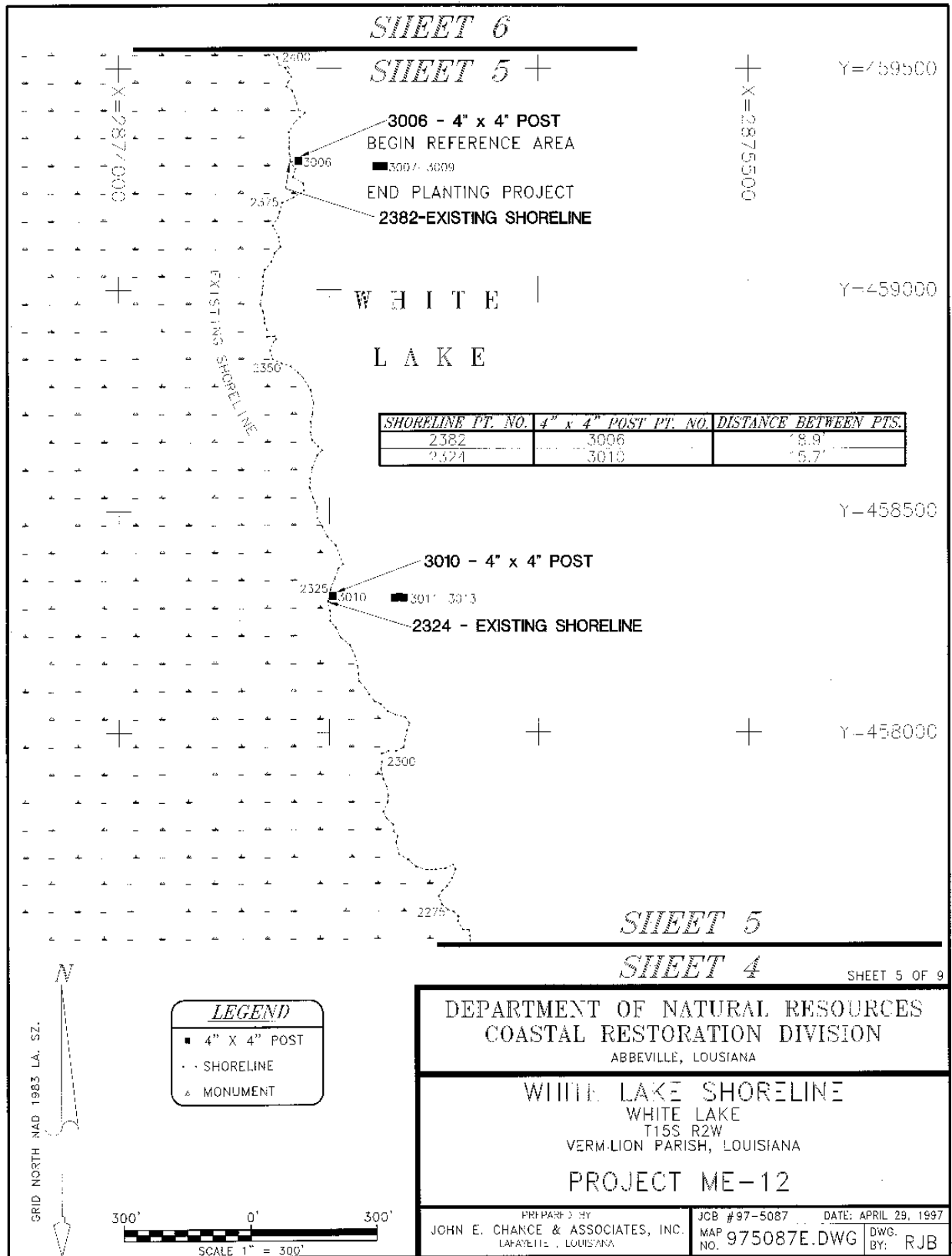
Figure A3. SW Shore White Lake Protection DEMO (ME-12) shoreline location survey showing station 5 (3010) and 6 (3006) in the project area, plant sampling location, and the distance from the shoreline marker to the existing shoreline.
