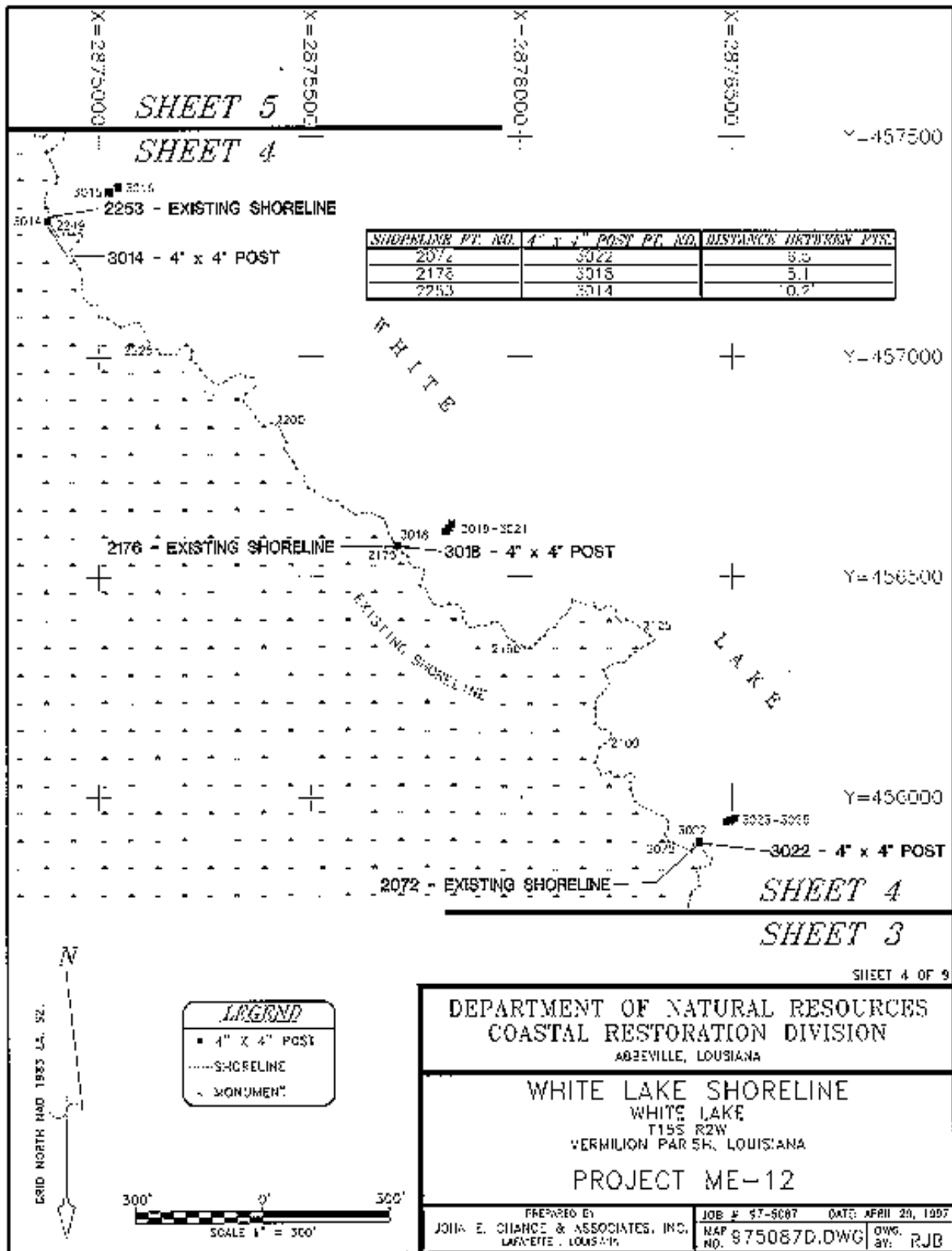
Figure A2. SW Shore White Lake Protection DEMO (ME-12) shoreline location survey showing station 2 (3022), 3 (3018), and 4 (3014) in the project area, plant sampling location, and the distance from the shoreline marker to the existing shoreline.
