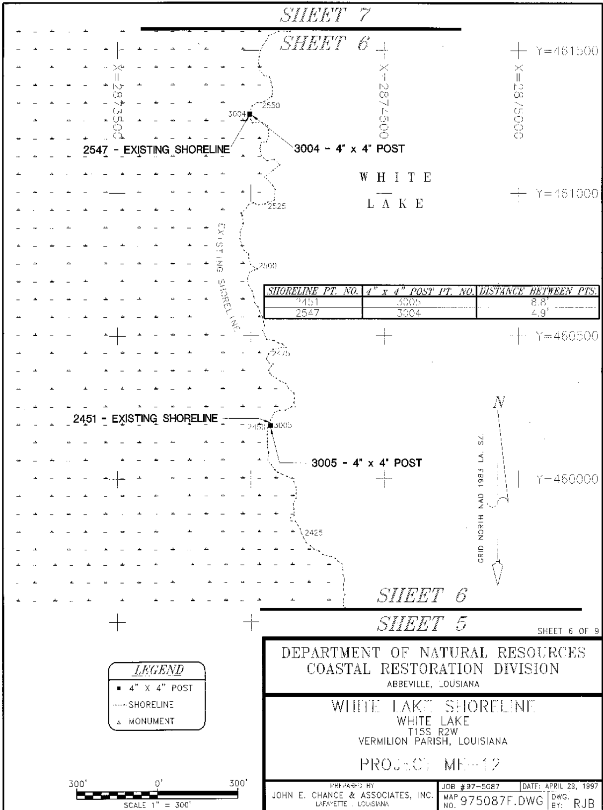
Figure A4. SW Shore White Lake Protection DEMO (ME-12) shoreline location survey showing station R-1 (3005) and R-2 (3004) in the reference area and the distance from the shoreline marker to the existing shoreline.
