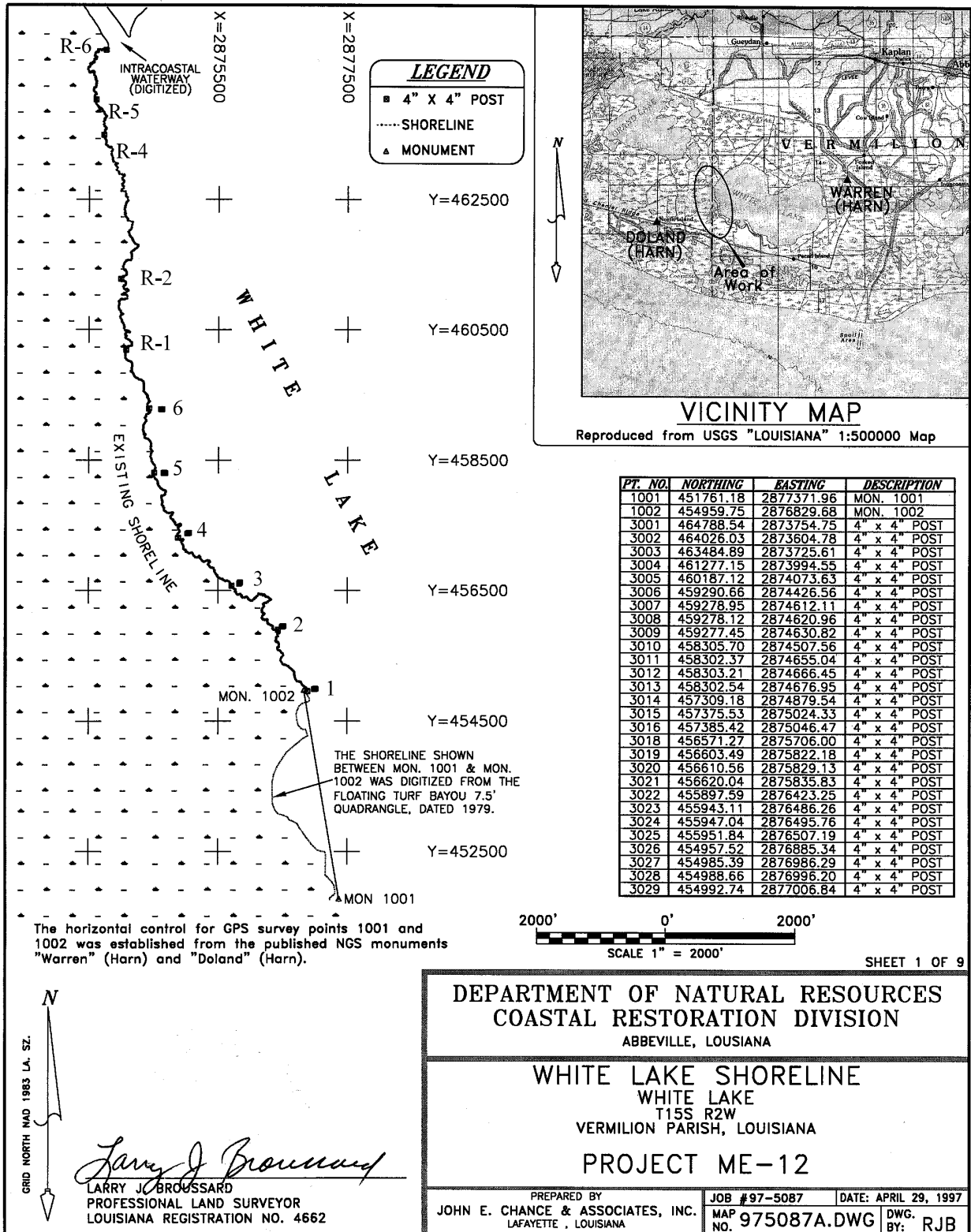
Figure 2. SW Shore White Lake Protection DEMO (ME-12) plan view showing the project and reference area.
