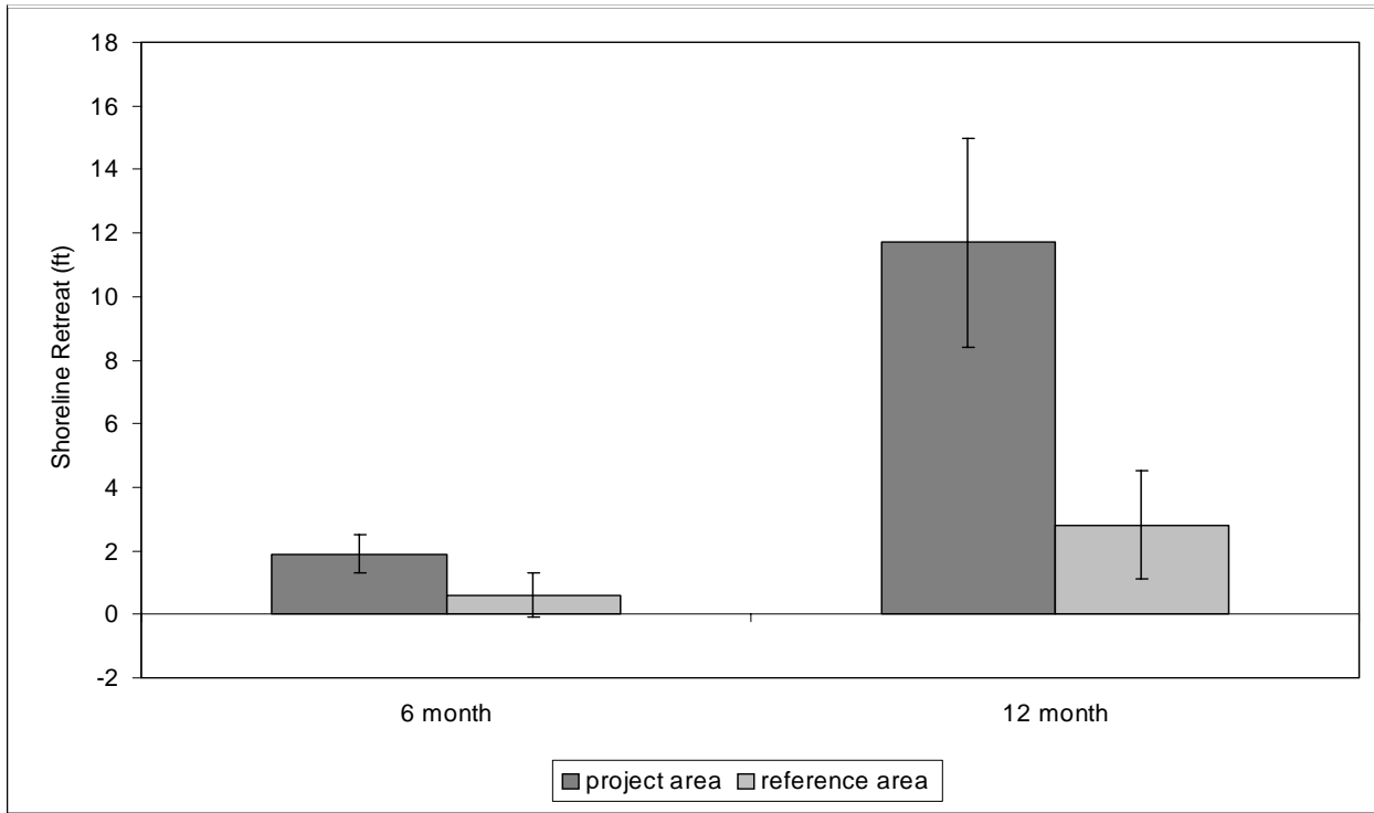
Figure 5. SW Shore White Lake Protection DEMO (ME-12) showing shoreline retreat (feet) in the project and reference area at the 6 and 12 month sampling period.
