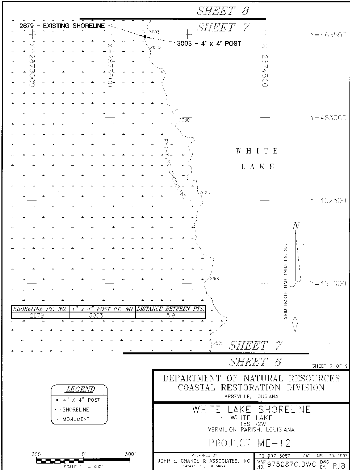
Figure A5. SW Shore White Lake Protection DEMO (ME-12) shoreline location survey showing station R-4 (3003) in the reference area and the distance from the shoreline marker to the existing shoreline. Station R-3 was missing at the time of the survey.
