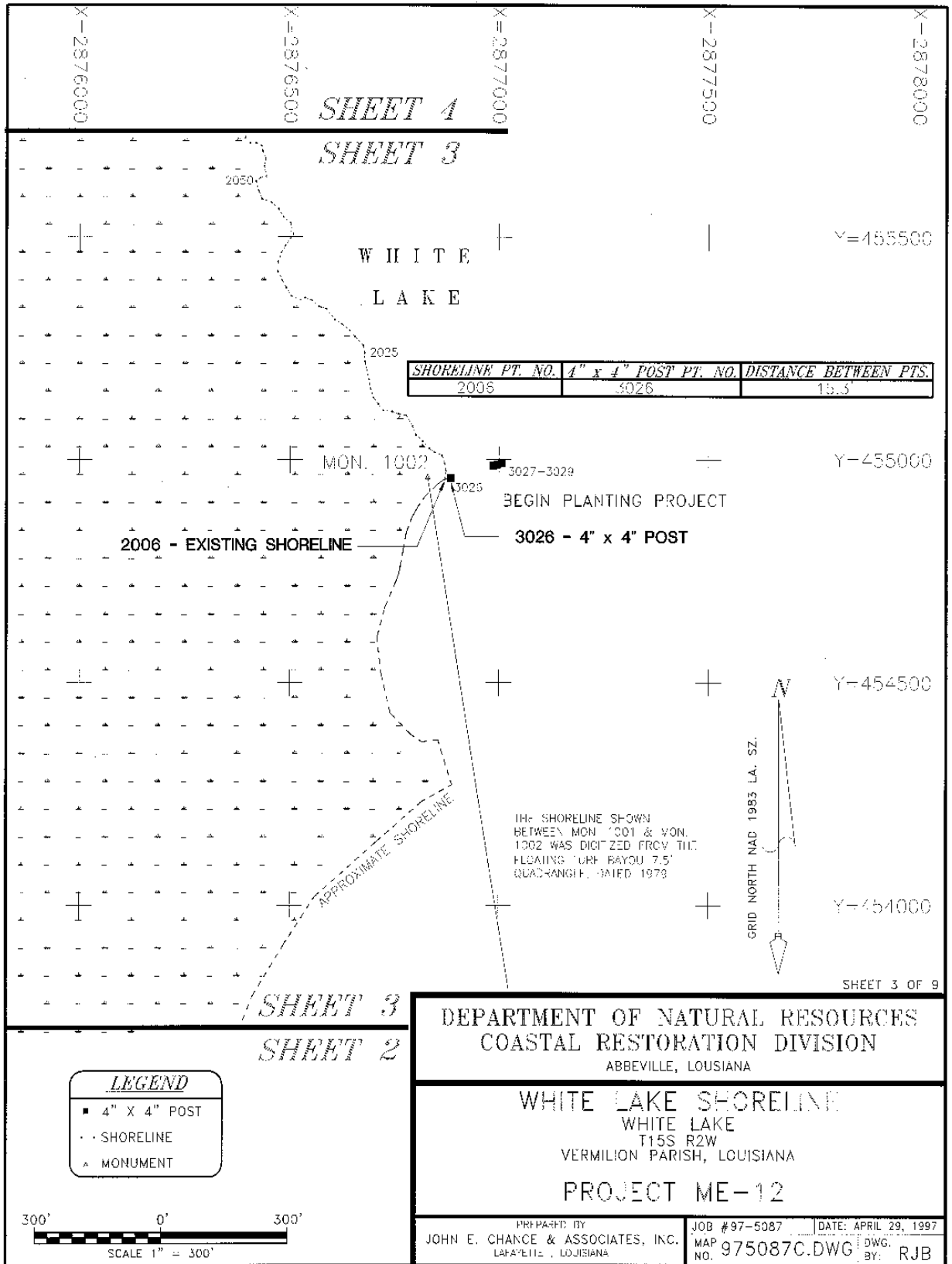
Figure A1. SW Shore White Lake Protection DEMO (ME-12) shoreline location survey showing station 1 (3026) in the project area, plant sampling location, and the distance from the shoreline marker to the existing shoreline.
