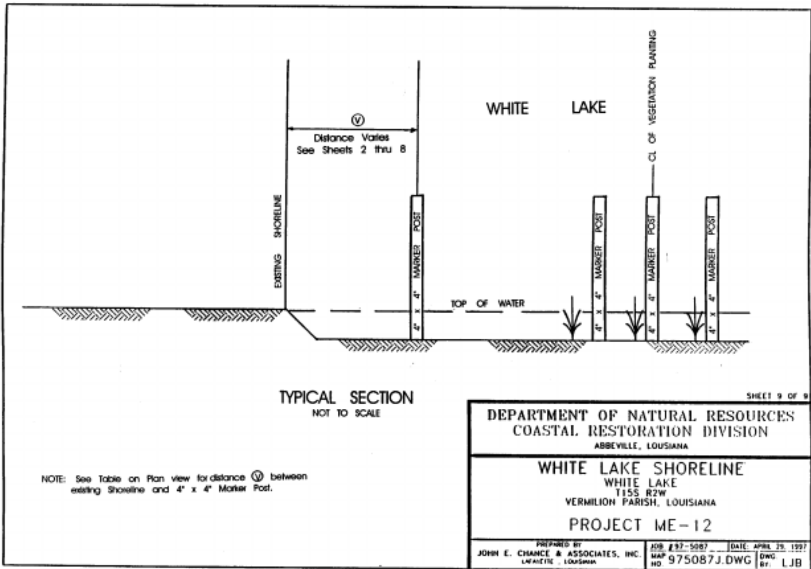
Figure 3. SW Shore White Lake Protection DEMO (ME-12) typical section showing existing shoreline, marker posts where direct measurements were taken, and location of plantings.
