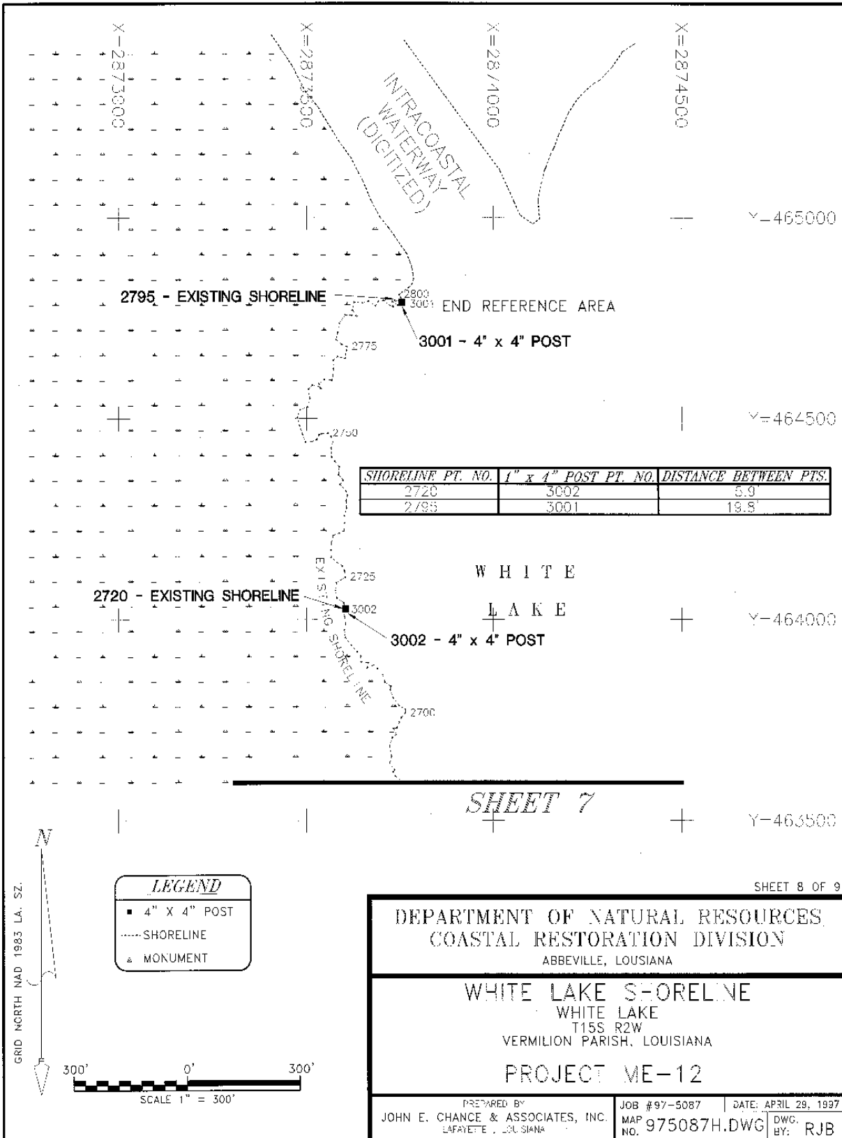
Figure A6. SW Shore White Lake Protection DEMO (ME-12) shoreline location survey showing station R-5 (3002) and R-6 (3001) in the reference area and the distance from the shoreline marker to the existing shoreline.
