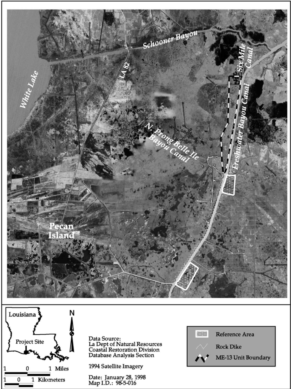
Figure 1. Freshwater Bayou Canal Bank Stabilization (ME-13) project area map showing project and reference area boundaries and rock dike location.
