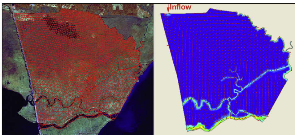
Fig. 9. The finite element mesh of the EJW used in the TABS-MD hydrologic model (left panel) and water flow vectors at steady state resulting from TABS-MD hydrologic model (right panel). See text for discussion.
