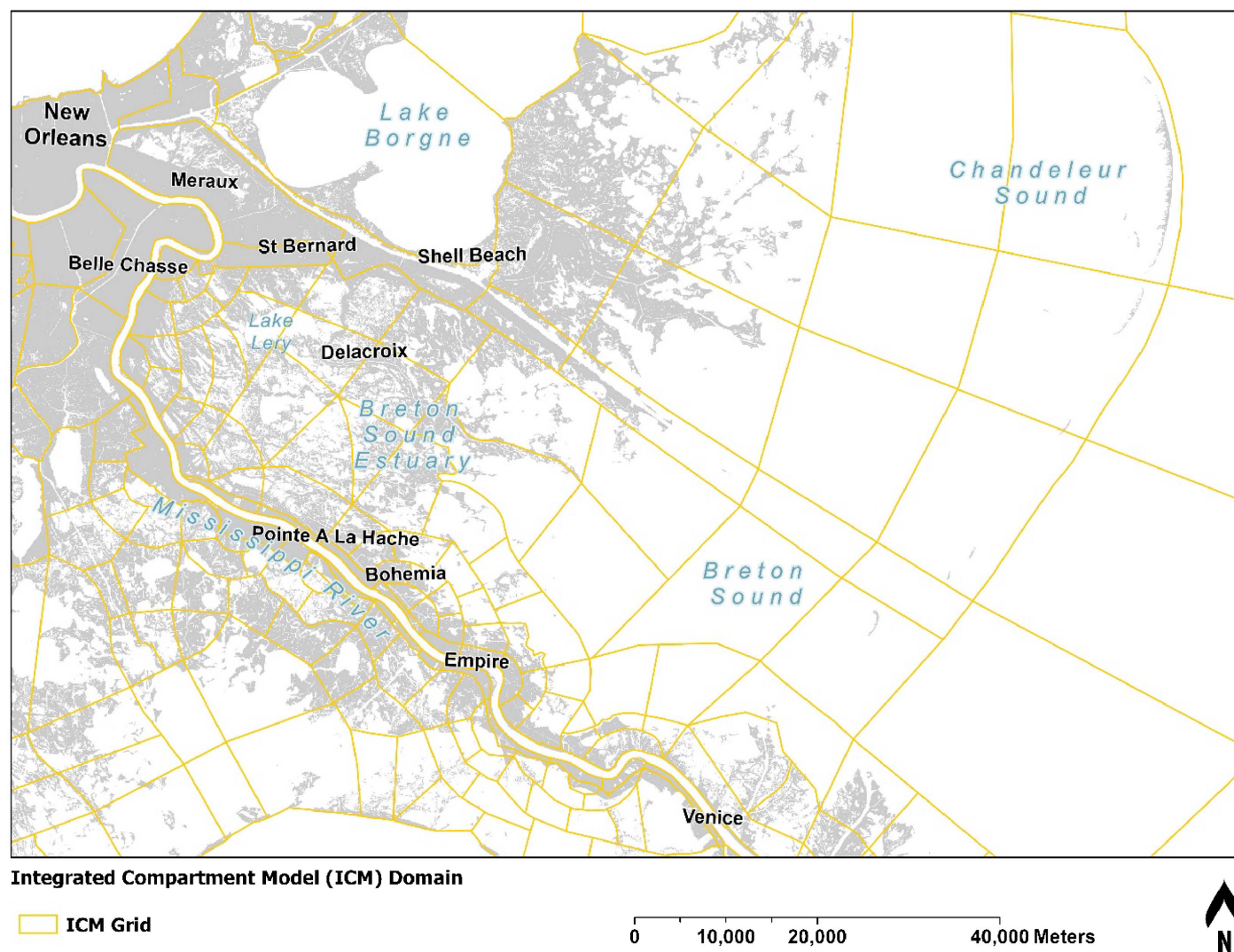
Fig. 3. Model grid/compartiment design for the ICM for the Breton Sound region. The compartment size in the area of interest ranged from 1.8 to 218.7 km 2 .
