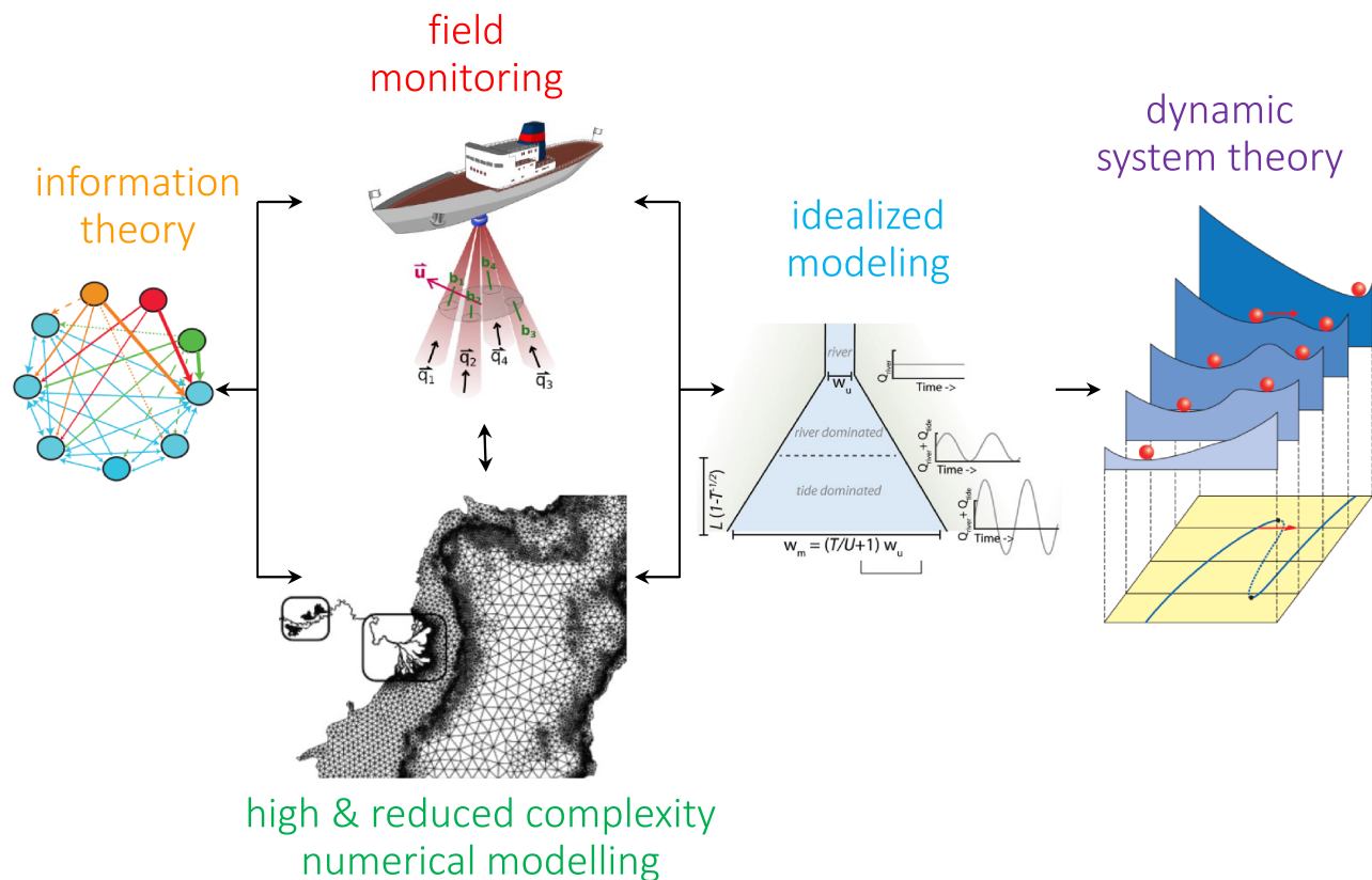
Figure 6. Synergy between alternative approaches to quantify morphodynamic stability of deltas. Field measurements are used to calibrate high-complexity models. In turn, modeling results help to optimize a monitoring plan. Information theory can be applied to test the degree in which high-complexity models correctly represent the information exchange between field stations in a delta. Using the collective understanding inferred from field observations and complex models, idealized or simplified models can be set up that capture basic mechanisms that can lead to instability. When the key mechanisms are understood, dynamic system theory can be employed to identify thresholds for regime shifts and to develop early warning indicators. Graphs obtained from Sendrowski and Passalacqua (2017) Sassi, Hoitink, de Brye, et al. (2011), Vermeulen et al. (2014), Nienhuis et al. (2018), and Scheffer (2009).
