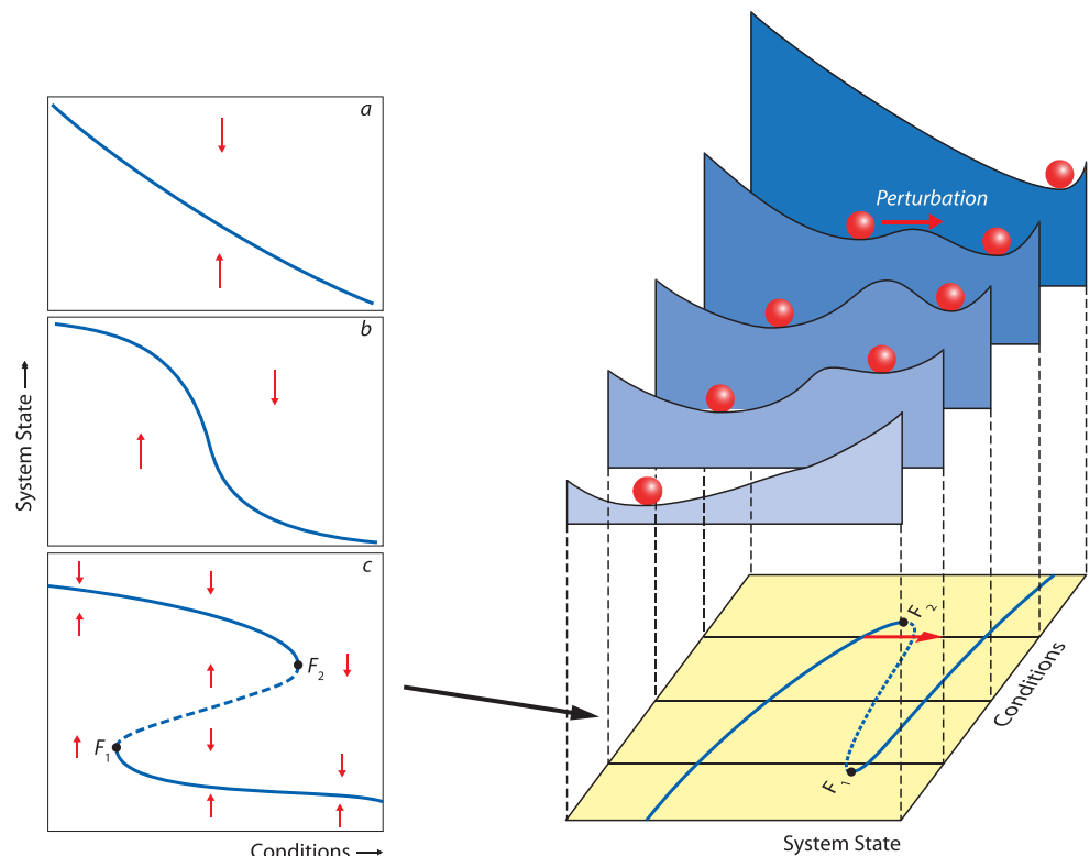
Figure 5. Regime shifts in deltas may be interpreted as critical transitions in a fold system. (a–c) Curves depict equilibrium conditions as a function of forcing conditions. If the curve is folded, as in (c), alternative equilibria exist for the same conditions. The arrows illustrate in which direction the system moves if it is not in equilibrium, showing all curves to be stable except for the dashed line in (c). The dashed line can be interpreted as the border between two basins of attraction, as illustrated in the right figure. Adopted from Scheffer (2009).
