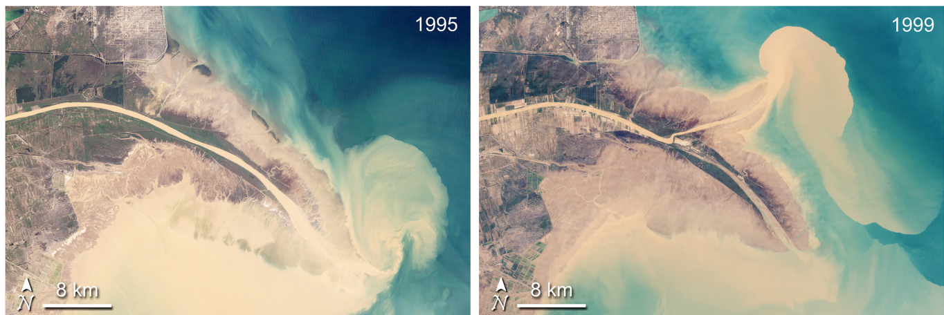
Figure 1. Scientific understanding about the natural process of avulsion has laid the basis for large-scale human interventions. In the Yellow River Delta, illustrated here, a human-induced avulsion occurred between 1995 and 1999. Image courtesy: NASA Earth Observatory.
