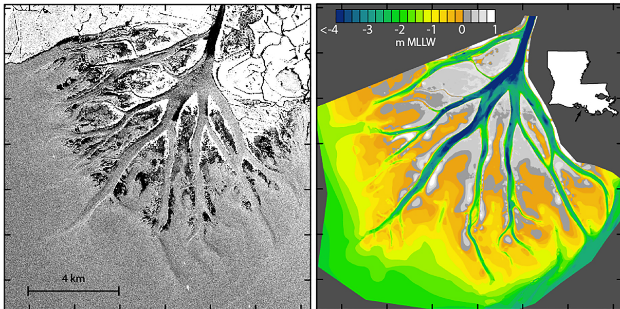
Figure 3. Airborne radar allows to monitor shallow bathymetry at high-resolution, complementing shipborne hydrographic surveys. (left) Image of Wax Lake Delta from an uninhabited aerial vehicle synthetic aperture radar (6 May 2015). (right) Corresponding image based on a single-beam sonar survey (February 2015). MLLW abbreviates Mean Lower Low Water. Adjusted from Shaw et al. (2016).
