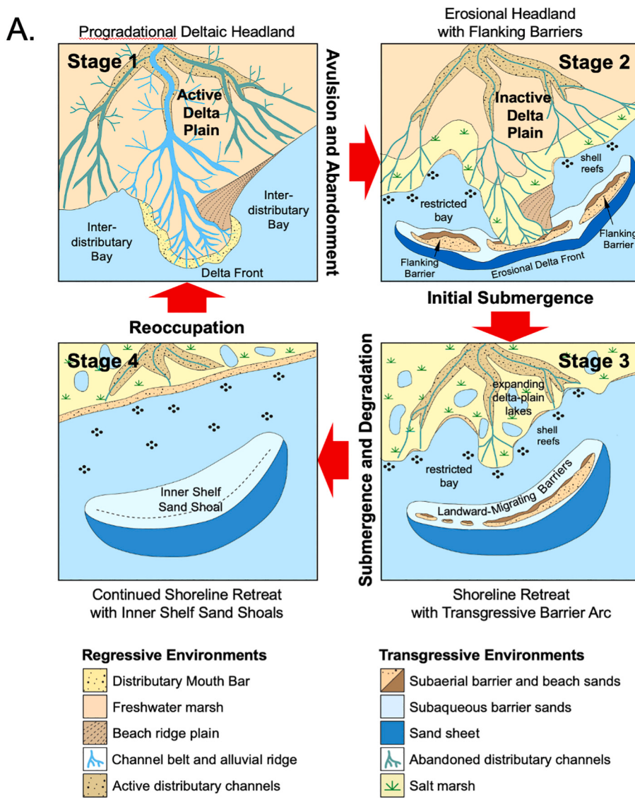
Fig. 3. The delta cycle concept (redrawn and modified from Penland et al., 1988, Blum and Roberts, 2012, and earlier work), illustrating the autogenic evolution of deltaic headlands following avulsion and relocation of feeder distributary channels. (a) Map views of changes through time in morphology and environments as a deltaic headland degrades. (b) Trends in deltaic headland area, shoreline length and other characteristics as deltaic headlands form then decay over time, with the state of individual MRD Holocene deltaic headlands as shown.
