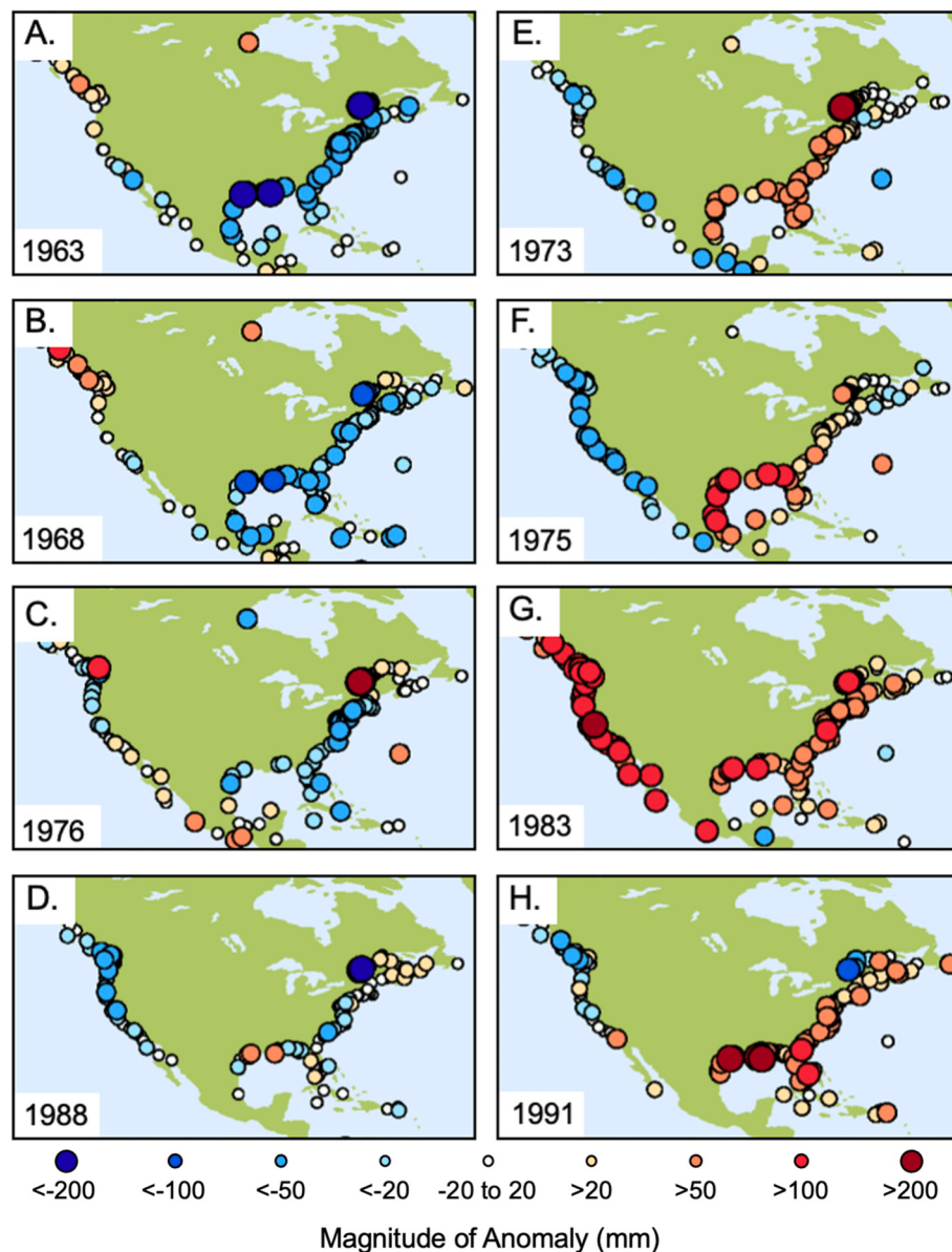
Fig. 10. Regional-scale annual anomalies in MSL for the years indicated from tide-gauge data in North America. (a to d) Negative annual MSL anomalies in the Gulf of Mexico. (e to h) Positive annual anomalies in MSL in the Gulf of Mexico. Each map represents departures for that tide-gauge station from the mean for the period 1960–1990. Maps obtained from the UK Permanent Service for Mean Sea Level (PSMSL) at https://www.psmsl.org .
