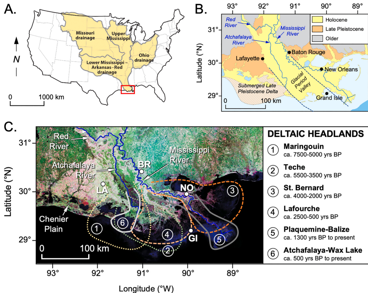
Fig. 1. (a) General location of the Mississippi River Delta study area, illustrating the Mississippi River contributing drainage basin. Red box indicates location of (b) and (c). (b) Generalized geologic map illustrating distribution of late Pleistocene and Holocene environments of deposition. (c) 2014 Landsat image with polygons that illustrate the general location and extent of major deltaic headlands that comprise the MRD. Modified from Blum and Roberts (2012) and references therein. (For interpretation of the references to colour in this figure legend, the reader is referred to the web version of this article.)
