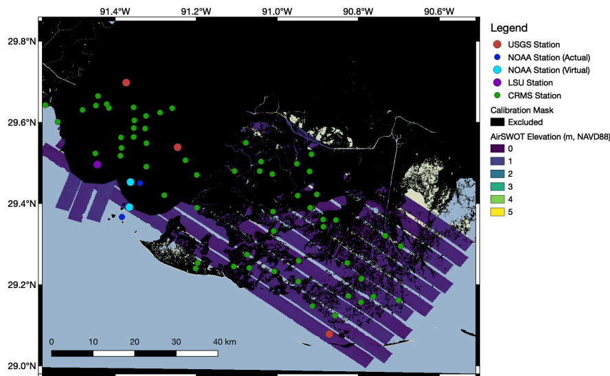
Figure 4. The areas that were excluded from the cross-track slope removal objective of the calibration procedure are shown in black. In the remaining non-masked areas, the calibration attempts to minimize the cross-track elevation slope with respect to the NAVD88 geoid.
