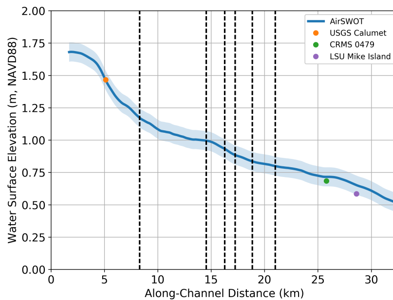
(a) WSE Profile for 9 May
