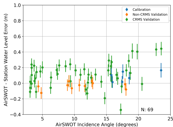
Figure 8. AirSWOT water level error vs. AirSWOT incidence angle. The error is shown as AirSWOT WSE minus in situ WSE. The points are colored according to the type of water level station as shown in the legend.
