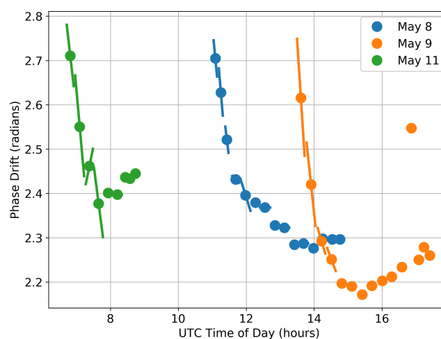
Figure 5. Phase drifts estimated by our calibration procedure for each day of the AirSWOT campaign. Early in each flight the estimated phase bias changes rapidly, but becomes more stable over time.
