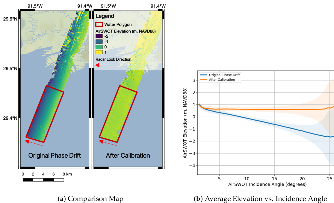
Figure 3. Comparison of AirSWOT elevation before and after applying our calibration method. Figure 3a shows maps of AirSWOT elevations using the original phase drift parameters (left map) and after applying our calibration method (right map). Figure 3b shows AirSWOT elevation vs. incidence angle for the water polygons (red boxes) in Figure 3a. The solid lines show the mean AirSWOT elevation at each incidence angle, while the shaded region shows \pm 1\sigma around the mean. After our calibration procedure, the anomalous cross-track slope seen in the original results has been corrected.
