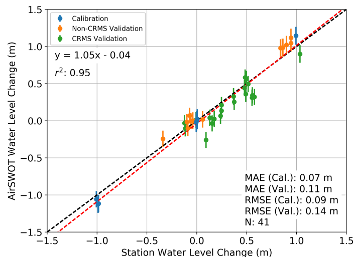
Figure 10. AirSWOT vs. in situ relative water level change, excluding CRMS stations at AirSWOT incidence angles of \geq 15^\circ . The points are colored according to the type of water level station as shown in the legend. The dashed black line is y = x . The dashed red line is a linear fit applied to all station types, with equation and r^2 as shown on the plot.
