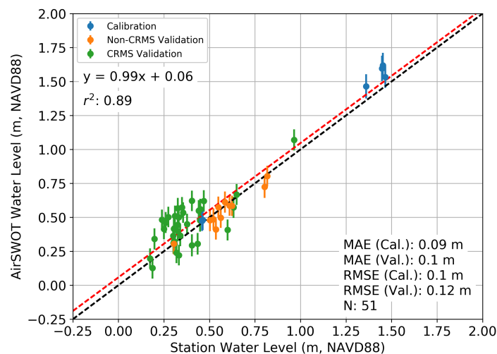
Figure 9. AirSWOT vs. in situ water level, excluding CRMS stations at AirSWOT incidence angles \geq 15^\circ . The points are colored according to the type of water level station as shown in the legend. The dashed black line is y = x . The dashed red line is a linear fit applied to all station types, with equation and r^2 as shown on the plot.
