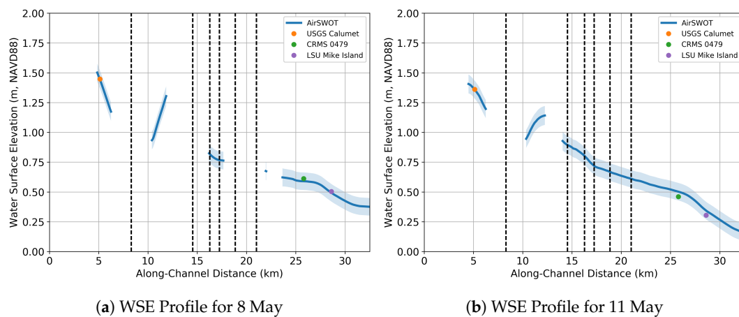
Figure 12. AirSWOT WSE profiles for 8 May (Figure 12a) and 11 May (Figure 12b) showing the effects of “dark water” on AirSWOT WSE. “Dark water” results in void data and potential anomalies in the small, disconnected regions between the void data.
