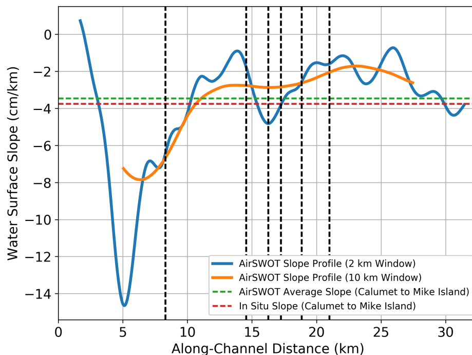
Figure 13. AirSWOT WSS profile for 9 May. The vertical dashed black lines represent major inflow and outflow locations along the channel. The solid blue and orange lines show the estimated AirSWOT WSS using different window sizes, while the dashed horizontal lines show the average slope between the Calumet and Mike Island stations as estimated by AirSWOT and the in situ data.
