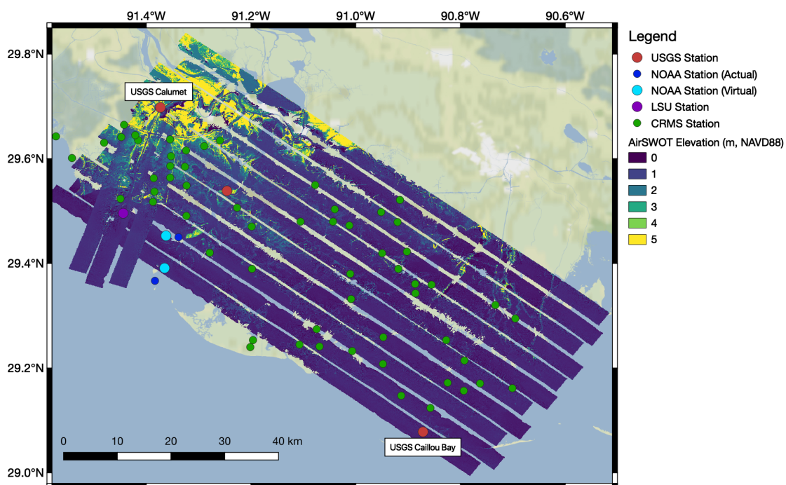
Figure 1. Overview map showing the locations of in situ water level stations overlaid on the AirSWOT elevation maps for 9 May 2015. The two stations used as GCPs in the AirSWOT calibration procedure are annotated with text labels. The background image is by Stamen Design, using OpenStreetMap data (see Acknowledgements).
