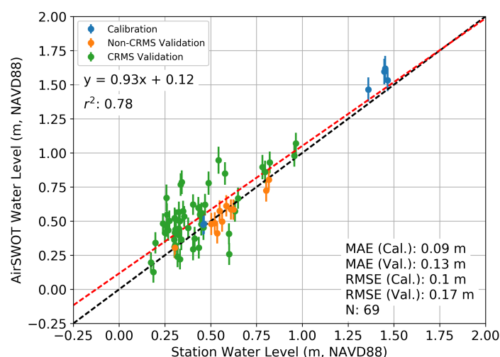
Figure 7. AirSWOT vs. in situ water level. The points are colored according to the type of water level station as shown in the legend. The dashed black line is y = x . The dashed red line is a linear fit applied to all station types, with equation and r^2 as shown on the plot.
