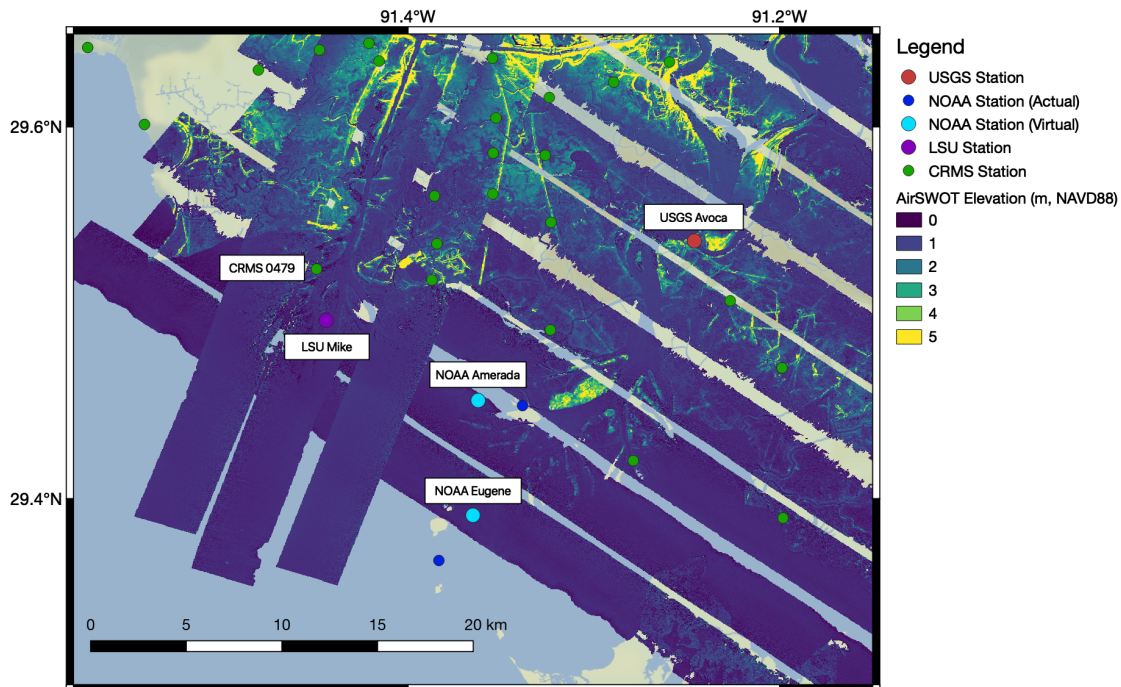
Figure 2. Map of the Wax Lake and Atchafalaya Deltas, showing the in situ water level station locations overlaid on the AirSWOT elevations for 9 May 2015. Some of the stations used for validation are annotated with text labels, for reference. The locations of the two NOAA stations were adjusted because their original positions were outside of the AirSWOT data extents. The background image is by Stamen Design, using OpenStreetMap data (see Acknowledgements).
